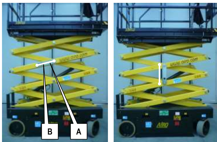
7-2: Lås af saks X10 EN, X10 EW, X10 EW-WIND, XS8 E RESTYLING LIGHT, XS8 E RESTYLING
