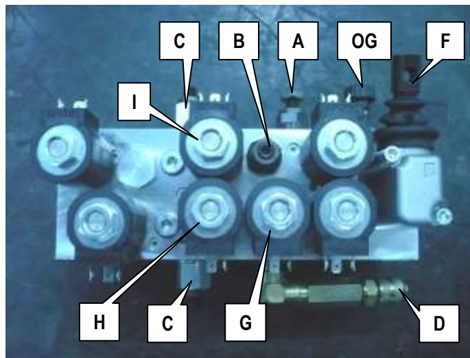
7-8: Hydraulikblok
