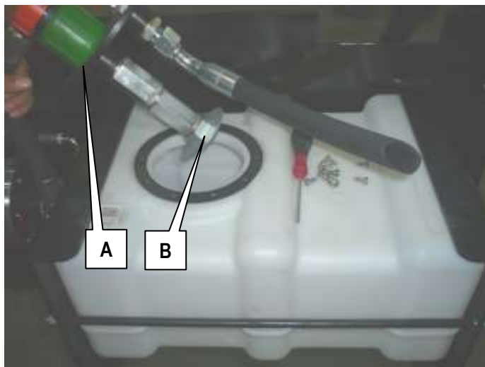
7-7: Tank X-serie
