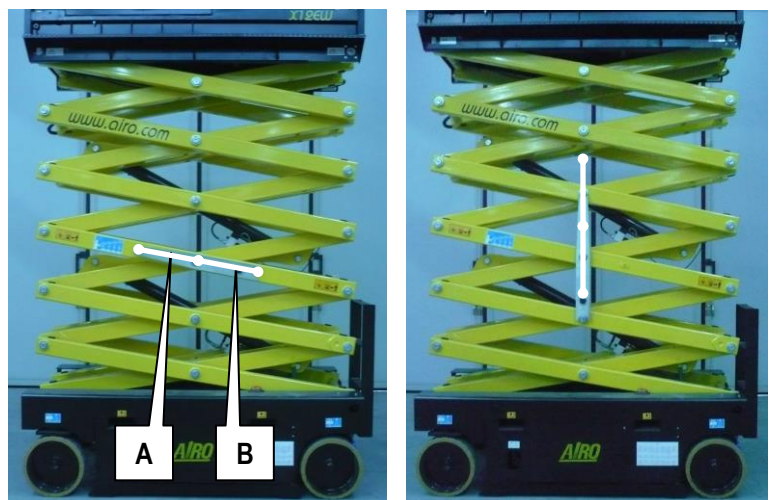
7-3: Scherensperrung X12 EN, X12 EW, X12 EW-WIND, X14 EW, XS9 E RESTYLING
