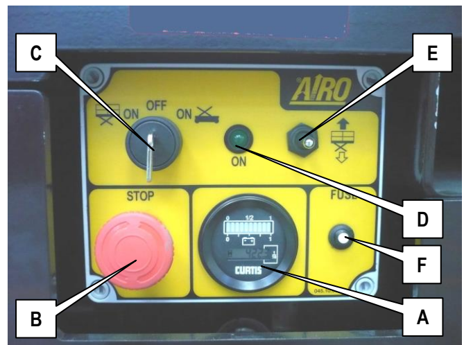
5-3: Bodenbedienpult
