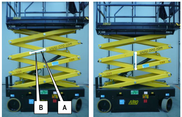
7-2: Scherensperrung X10 EN, X10 EW, X10 EW-WIND, XS8 E RESTYLING LIGHT, XS8 E RESTYLING
