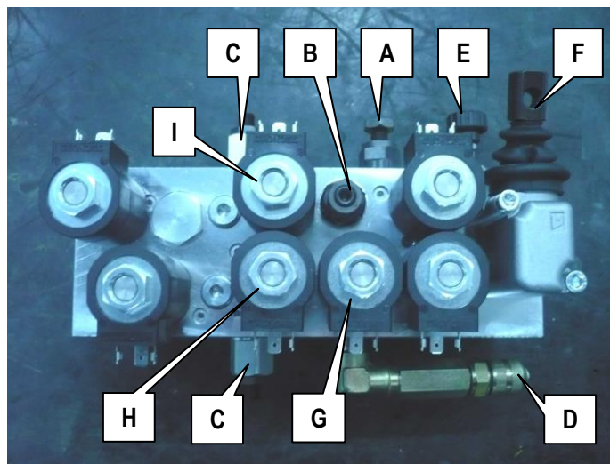
7-8: Hydraulikblock
