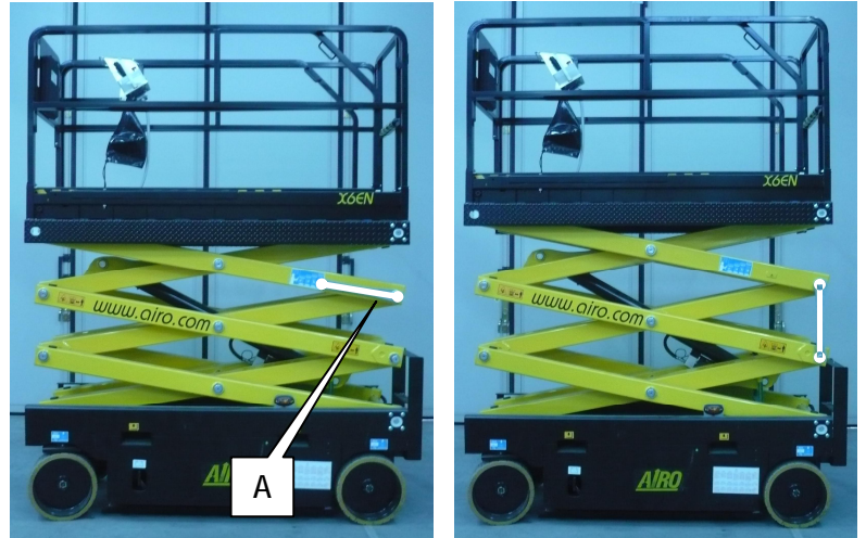
7-1: Blocage ciseaux X8 EN, XS7 E RESTYLING
