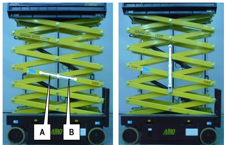
7-3: Blocage ciseaux X12 EN, X12 EW, X12 EW-WIND, X14 EW, XS9 E RESTYLING
