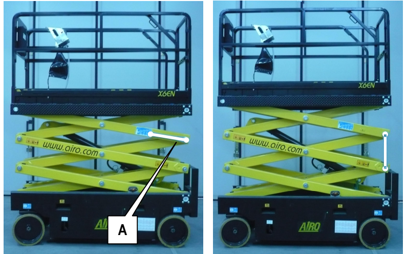
7-1: Blocage ciseaux X8 EN, XS7 E RESTYLING
