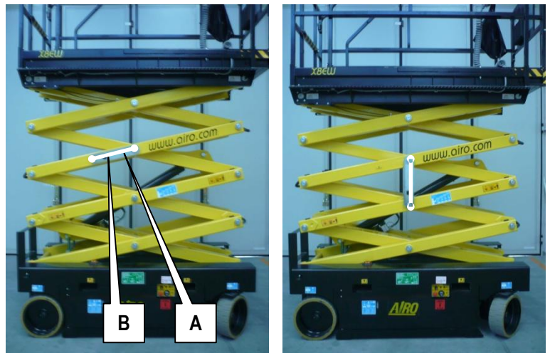
7-2: Blocage ciseaux X10 EN, X10 EW, X10 EW-WIND, XS8 E RESTYLING LIGHT, XS8 E RESTYLING
