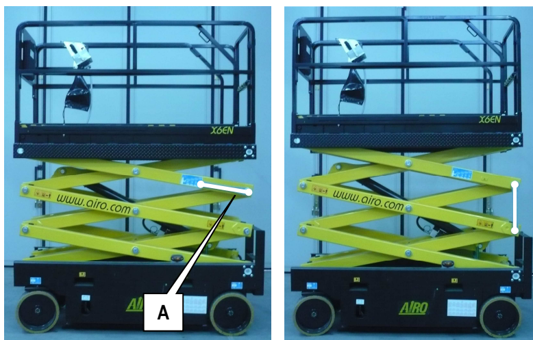
7-1: Blocage ciseaux X8 EN, XS7 E RESTYLING
