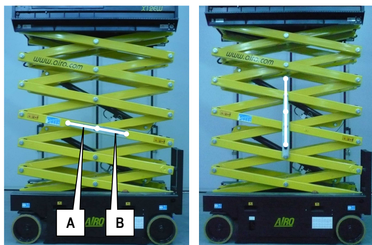
7-3: Blocage ciseaux X12 EN, X12 EW, X12 EW-WIND, X14 EW, XS9 E RESTYLING
