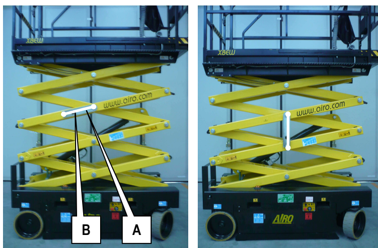
7-2: Blocage ciseaux X10 EN, X10 EW, X10 EW-WIND, XS8 E RESTYLING LIGHT, XS8 E RESTYLING
