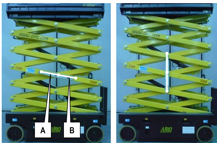
7-3: Blocare foarfecii X12 EN, X12 EW, X12 EW-WIND, X14 EW, X16 EW, X9 E RESTYLING
