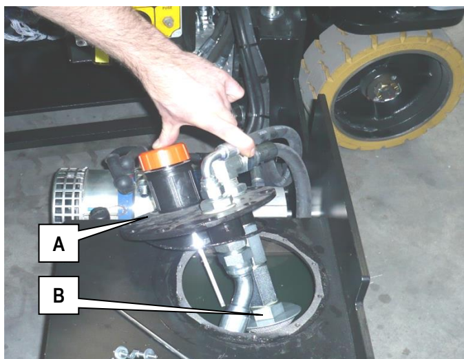
Rezervor seria XS E RESTYLING
